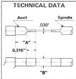
A = .600", B = .235"
