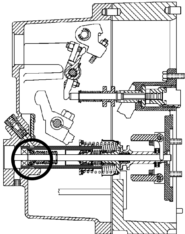
Typical 3406 Mechanical Governor
