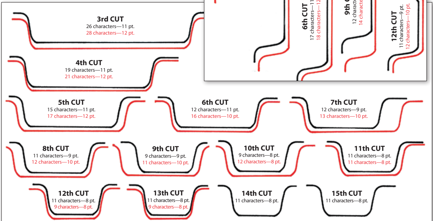
Bottom-Tab Style (actual size) Paper and Tyvek shown in black. Poly shown in red.
